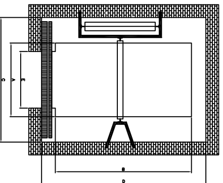
SHAFT TOP VIEW
